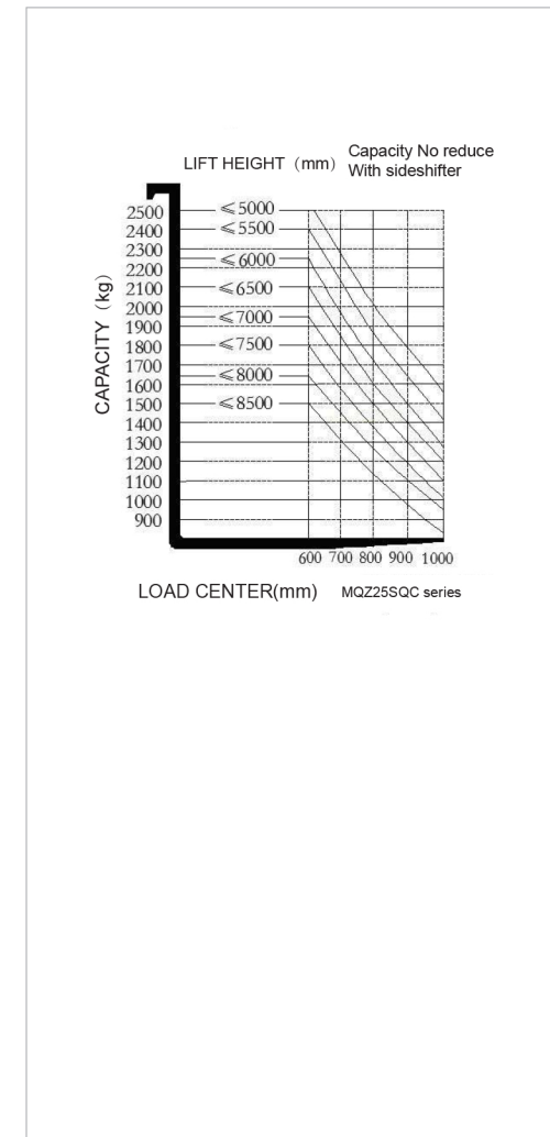
Load Chart
